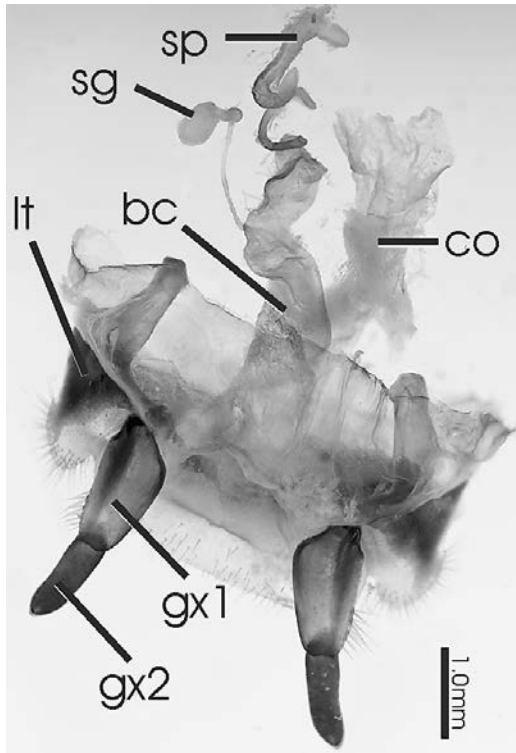
FIG. 3. Female reproductive tract of Sphodrosomus monteithi , ventral view. bc, bursa copulatrix; co, common oviduct; gx1, gonocoxite-1; gx2, gonocoxite-2; lt, laterotergite IX; sg, spermathecal gland; sp, spermatheca.
