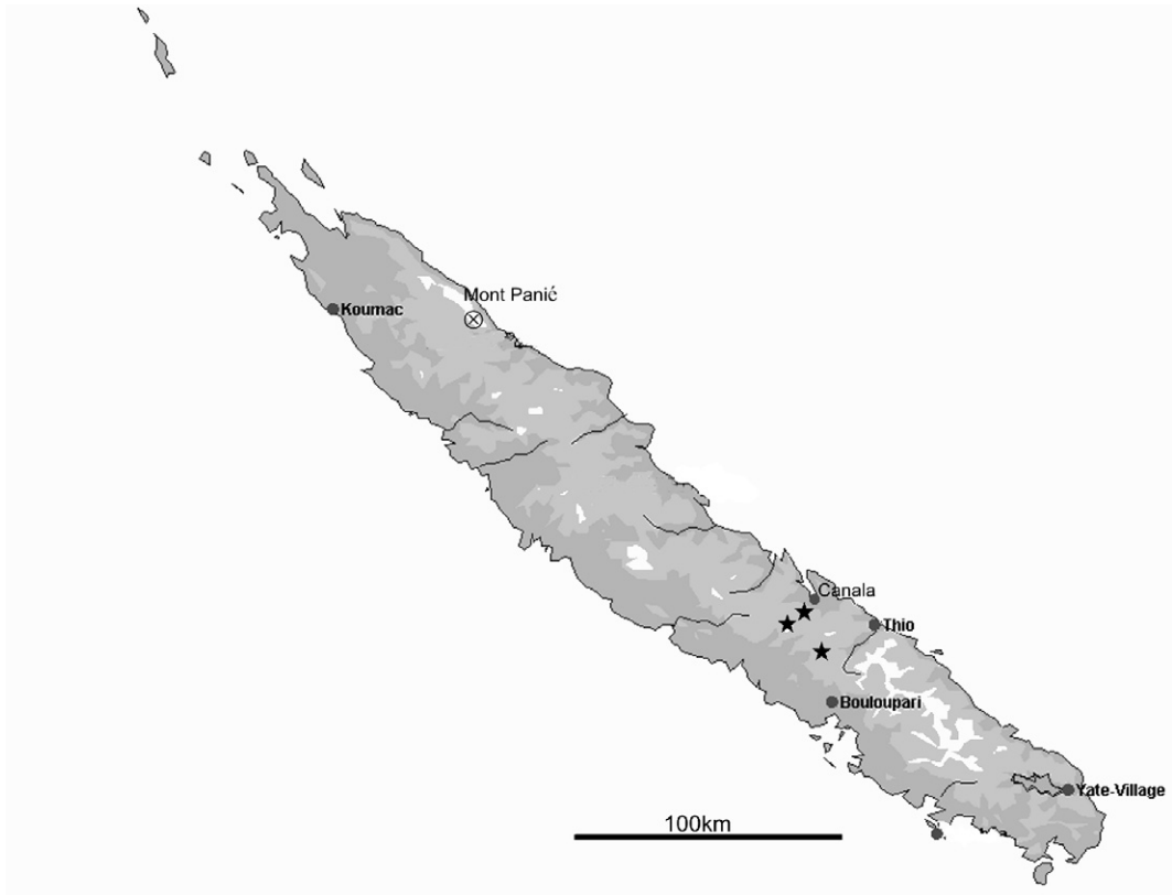
FIG. 5. Distribution of Sphodrosomus species. ⊗, S. monteithi . ★, S. saisseti .
